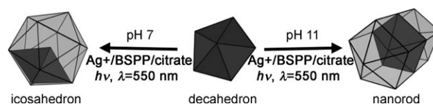
Figure 1. pH-dependent plasmon-mediated growth processes involving the photodeposition of Ag on plasmonic decahedral Au seeds. Au dark gray; Ag light gray.
